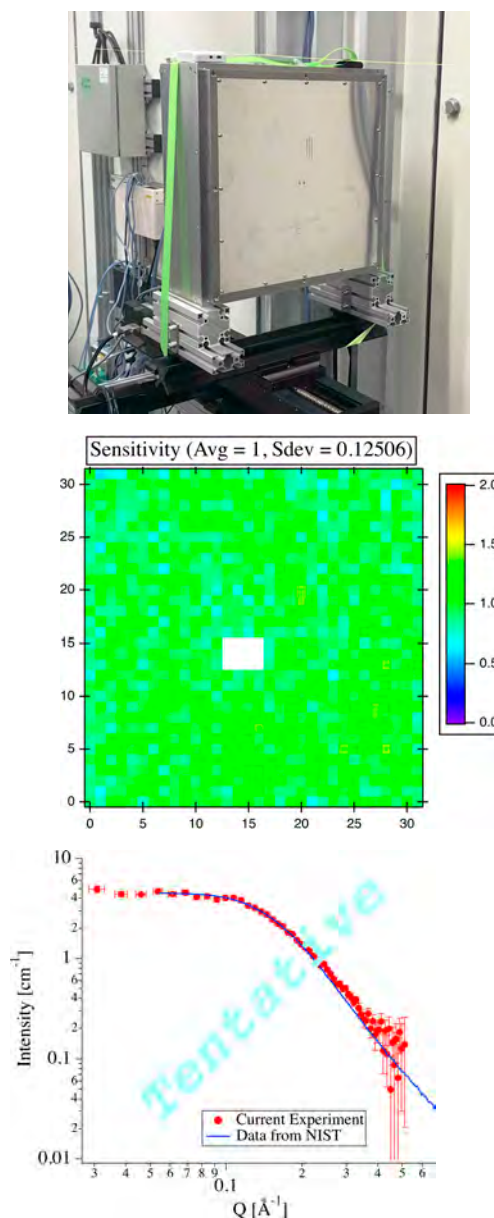
Figure 1. Top: a picture of the detector. Middle: the observed sensitivity of the detector. Bottom: the observed scattering profile of a glassy carbon as a standard sample compared with the data from NIST.
