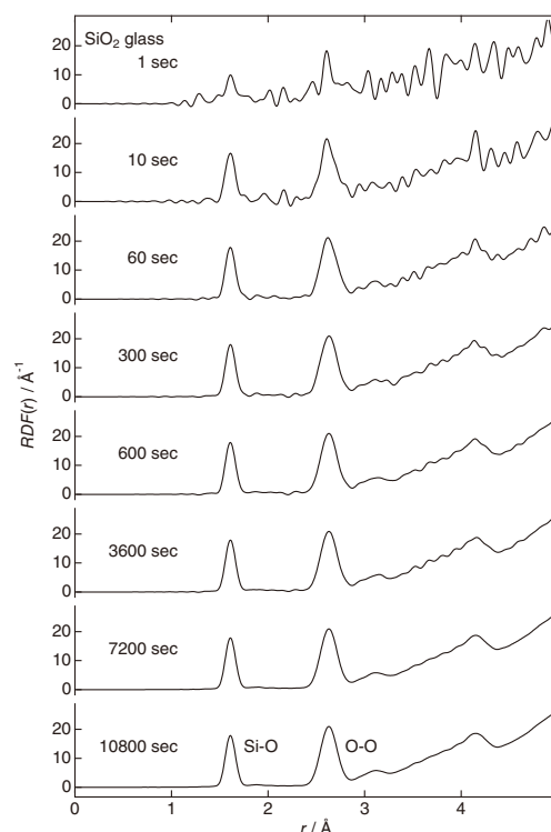
Figure 4. RDF(r) of SiO 2 glass rod measured from 1 sec to 3 h at 900 kW.
