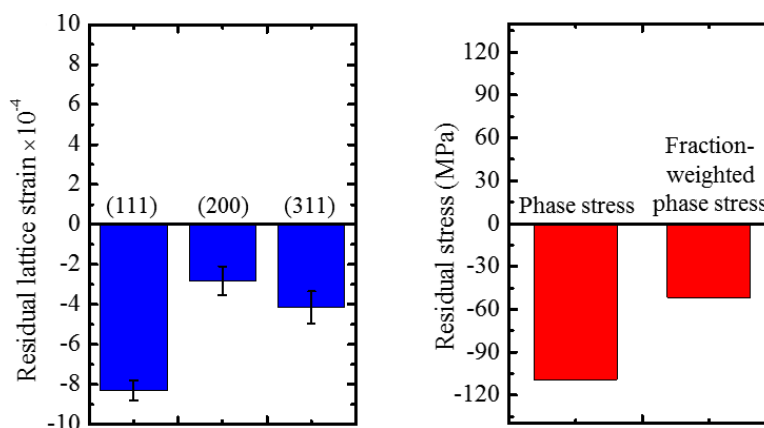
Figure 1. Residual phase lattice strain and stress in the unloaded state.
