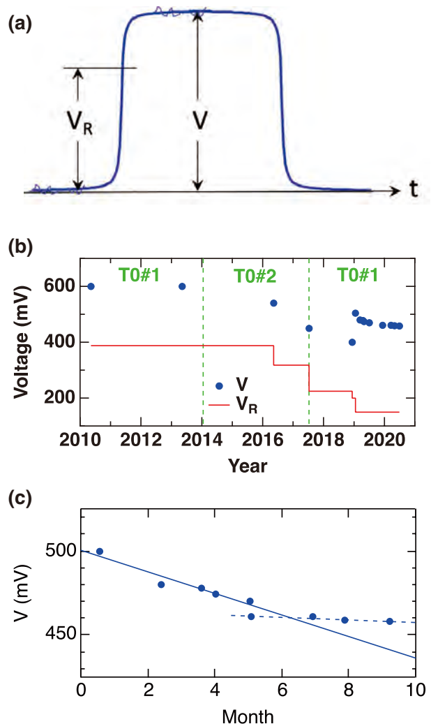
Figure 1. (a) Schematic drawing of the output voltage of the rotational signal as a function of time (t). (b) Variations of V and V_R . The T0 chopper in operation at the time is indicated. (c) Variation of V since January 1, 2019 (Month = 0) indicated by removing the beam off period.
