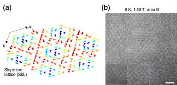
Figure 3. (a) Schematic illustration of the magnetic skyrmion on the kagome lattice of Gd_3Ru_4Al_{12} . (b) Real-space observation of the spin texture on the (001) plane of Gd_3Ru_4Al_{12} by Lorentz transmission electron microscopy. [cited from Ref. 10]
