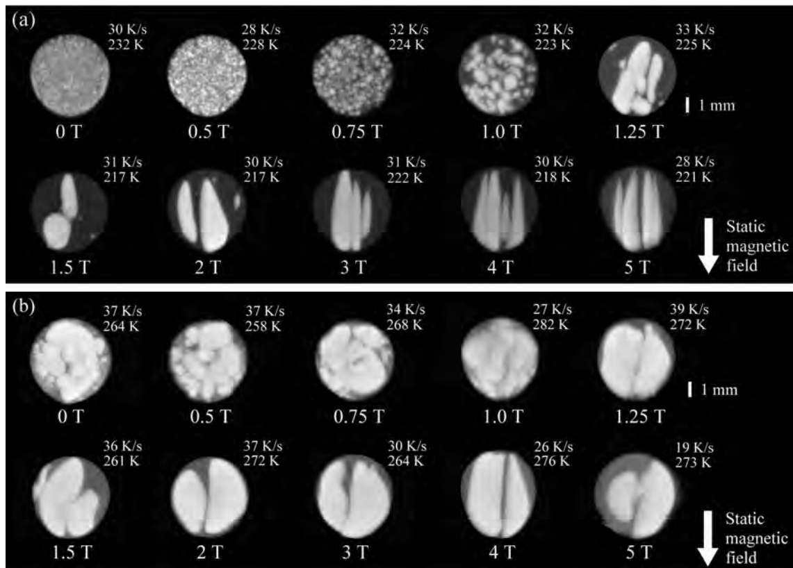
Figure 2. Phase separation structures in Cu-Co alloys solidified under different static magnetic fields obtained through neutron CT experiments. The brighter and darker regions indicate Co-rich and Cu-rich phases, respectively. The values in the upper right of each image represent the cooling rate and the degree of undercooling. (Adapted from Ref. 3)
