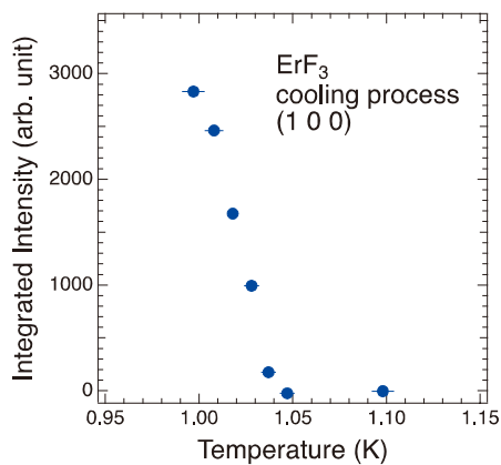
Figure 2. The temperature dependence of the magnetic peak intensity of \text{ErF}_3 .
