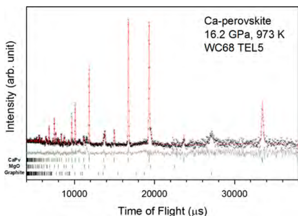
Figure 3. Observed (cross), calculated (red line) and difference (gray) for the profile of Ca-perovskite. Vertical bars indicate calculated positions for reflections of Ca-perovskite, MgO endcap and graphite capsule. The binning width of the data is \Delta t/t = 0.001 .
