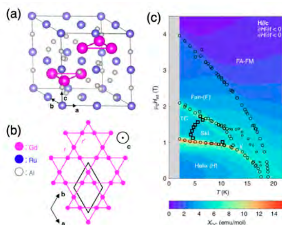
Figure 1. [(a), (b)] Schematic illustrations of the crystal structure of \text{Gd}_3\text{Ru}_4\text{Al}_{12} . (c) Magnetic phase diagram of \text{Gd}_3\text{Ru}_4\text{Al}_{12} for magnetic field along the c axis. Color scale shows the real part of ac magnetic susceptibility. [cited from Ref. 10]
