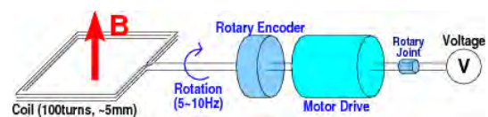
Figure 4. Concept of the search coil.
