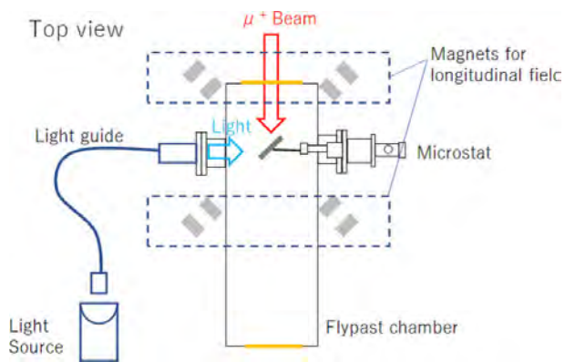
Figure 3. LF-μSR setup with light source.
