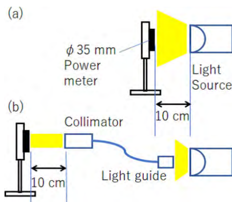
Figure 2. Setup for examining the pulse energy of the light source.
