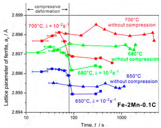
Figure 3. Change in lattice constants of ferrite during the thermomechanical processing (Fe-2Mn-0.1C, strain rate: 10^{-2} \text{ s}^{-1} ). Adapted from Ref. [4]. Reproduced with permission from Elsevier.
